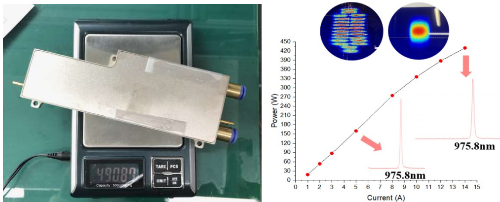
Figure 2. 420W@135μm NA0.22 LD.
