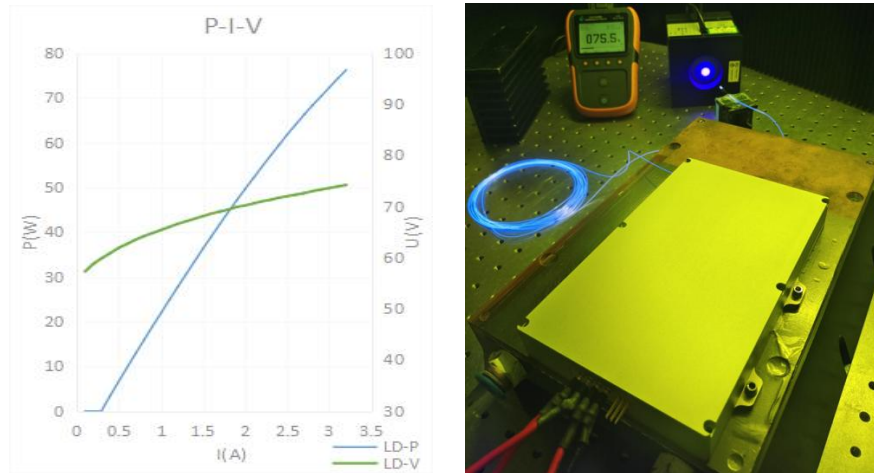
Figure 4. Power and voltage test data
