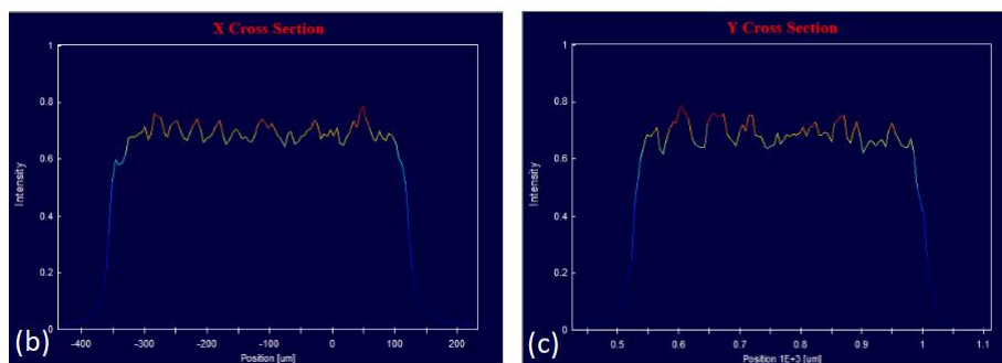
Figure 5. (a) 100\mu\text{m} \times 100\mu\text{m} square homogenized beam at end face of fiber (b) X cross section power distribution (c) Y cross section power distribution
